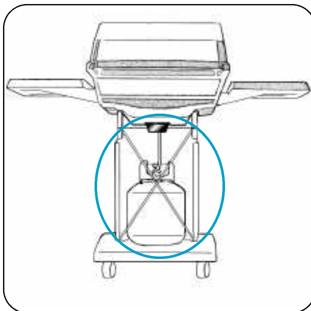
Rear view of Series 4000 grill with the X-Brace retainer wire shown in place.
